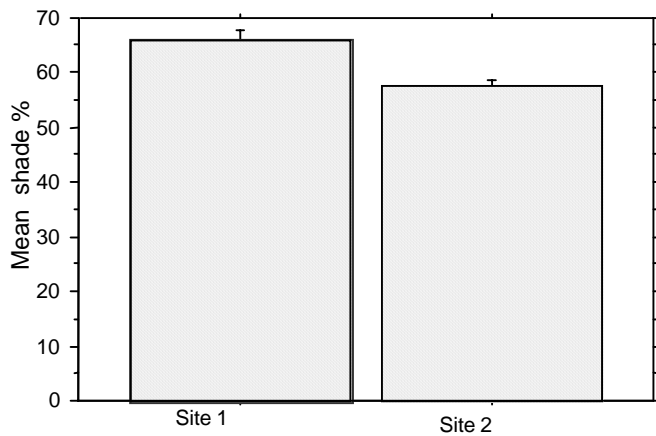
Figure 1. Mean percentage shade in Maesopsis -dominated site and Cinnamomum -dominated site
