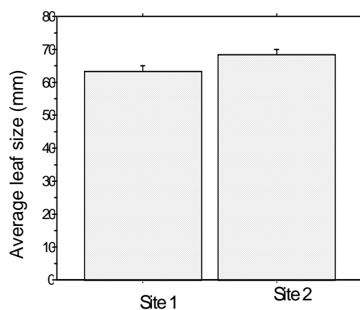
Figure 4. Average leaf length at site1 and site2.
