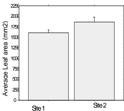
Figure 3. Average leaf area at site 1 and site2.
