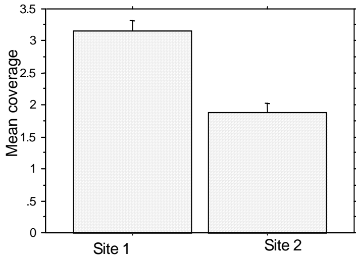
Figure 2. Mean coverage of L. camara between Maesopsis -dominated site and Cinnamomum -dominated site
