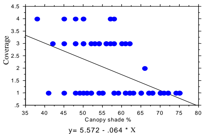
Figure 6. Relationship between cover of L. camara and percentage shading ( Cinnamomum -dominated site).
