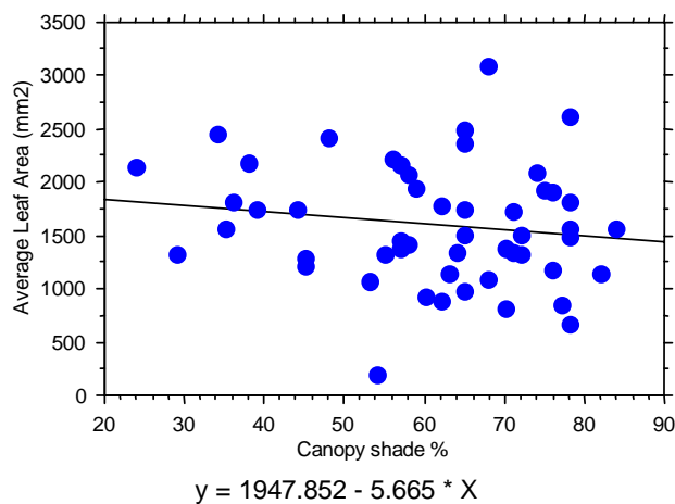
Figure 7. Relation between average leaf area and percentage shading ( Maesopsis -dominated site).
