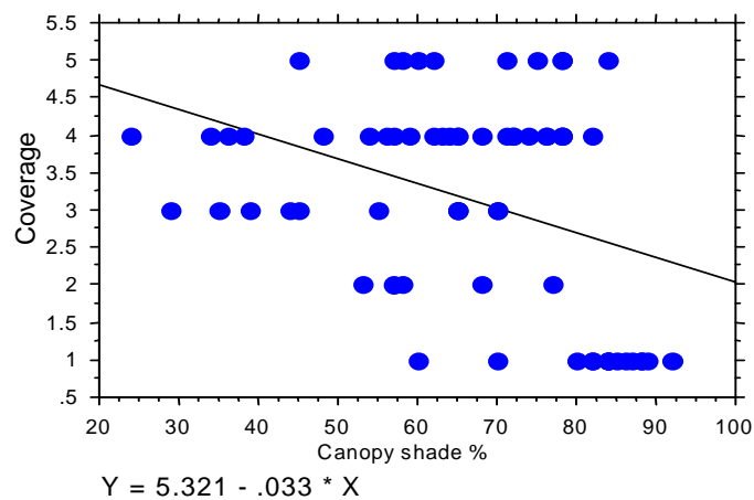
Figure 5. Relationship between cover of L. camara and percentage shading ( Maesopsis -dominated site).
