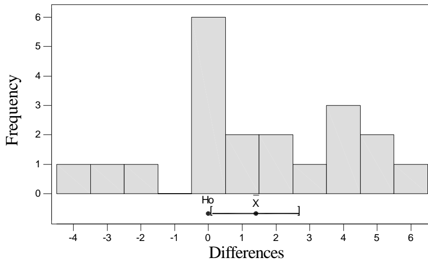
Figure 2. A comparison of family level richness between cut and uncut sites (cut quadrant richness minus uncut quadrant richness). N=20. All data collected from Amani floodplain, Tanzania.
