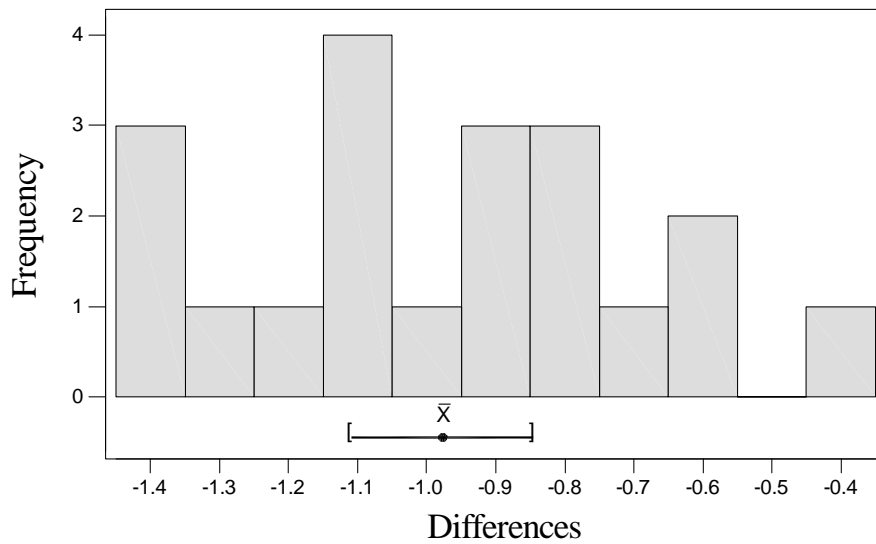
Figure 1. A comparison of family level diversity between cut and uncut sites (cut quadrant diversity minus uncut quadrant diversity). N=20. Shannon-Weiner index used to calculate diversity. All data collected from Amani floodplain, Tanzania.
