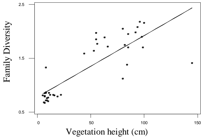
Figure 3. A correlation between vegetation height and family diversity; N=40 . Diversity calculated using the Shannon-Weiner index for data collected from Amani floodplain, Tanzania.
